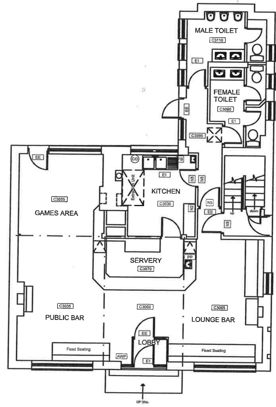
EXISTING GROUND FLOOR PLAN 2004 SCALE 1:50
