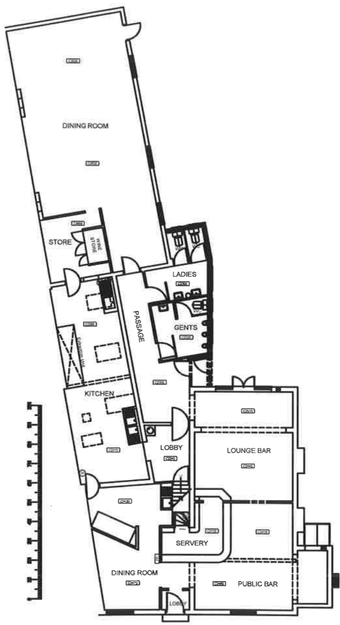
EXISTING GROUND FLOOR PLAN 2004 SCALE 1:100
