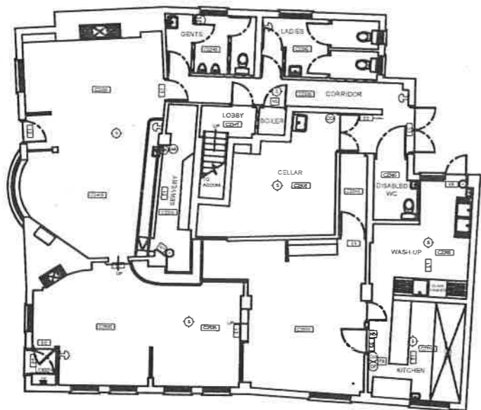
EXISTING GROUND FLOOR PLAN 2004 SCALE 1:100
