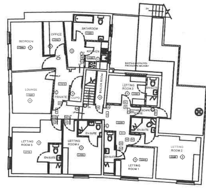
EXISTING FIRST FLOOR PLAN 2004 SCALE 1:100
